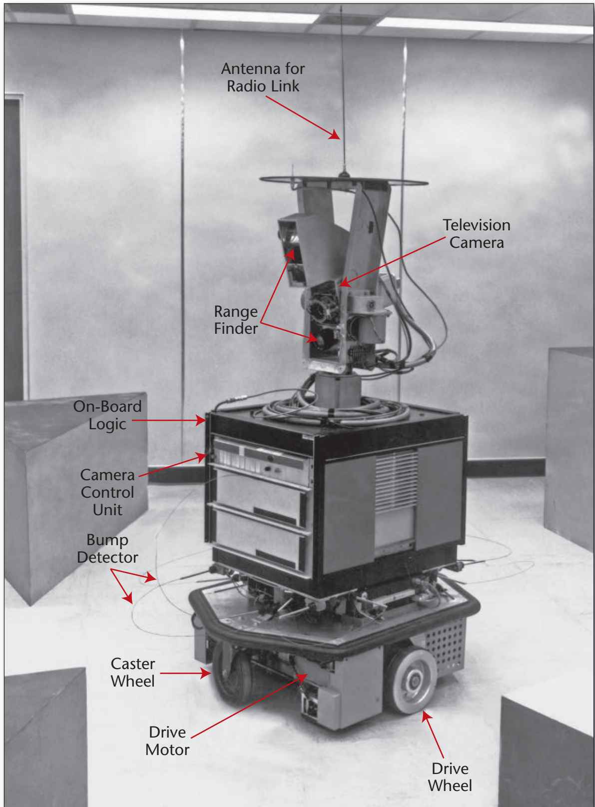
Figure 2. Shakey with Components Labeled.
