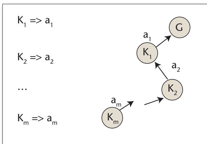
Figure 12. Teleo-Reactive Programs.
