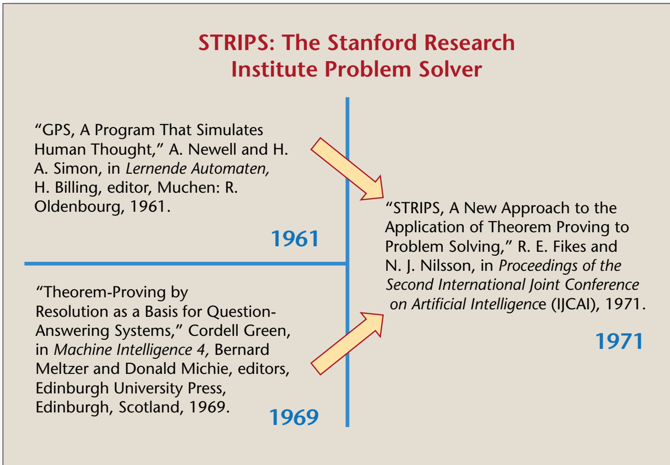
Figure 8. STRIPS.
